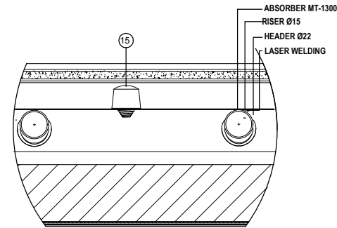
DETAIL G
